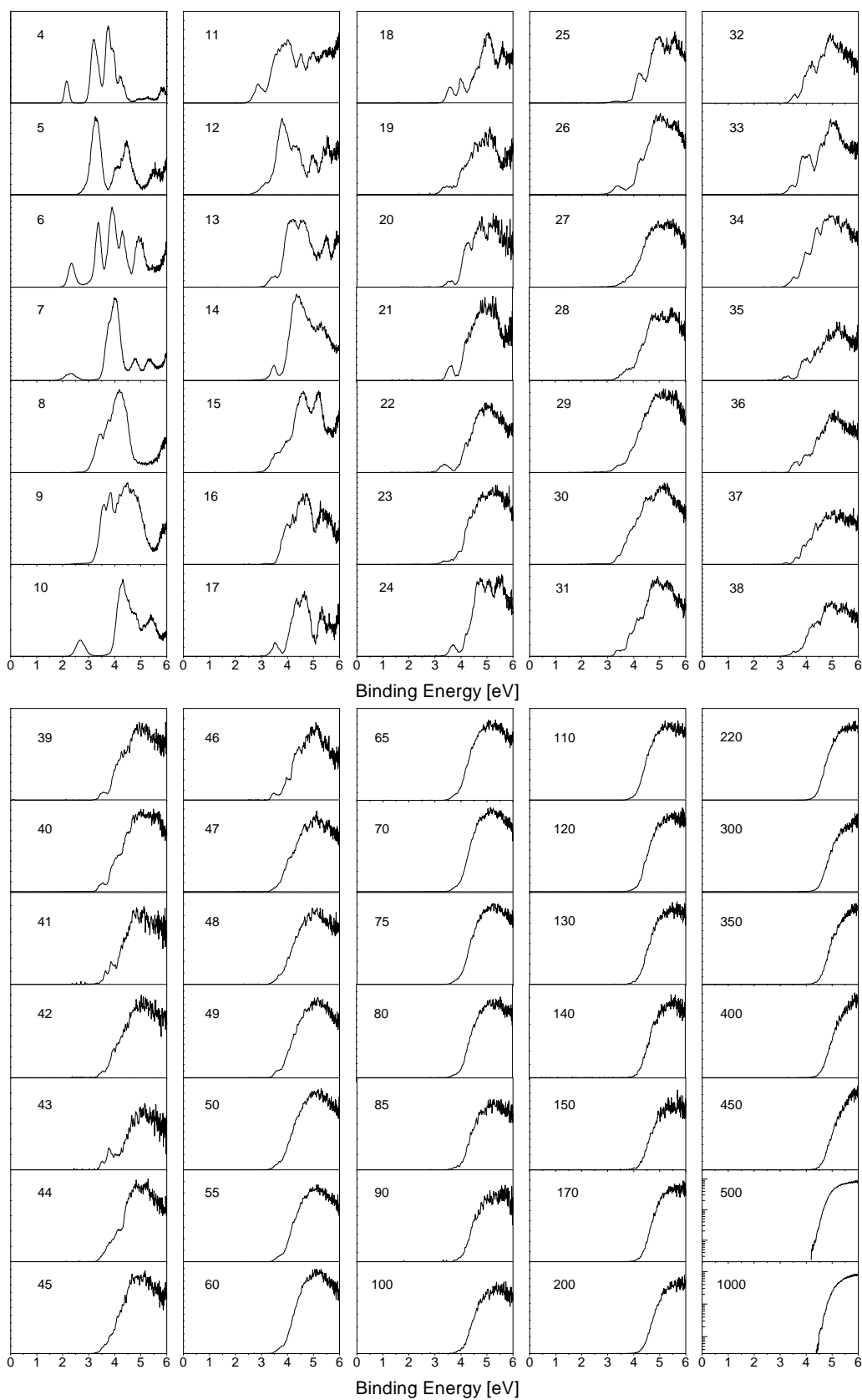
Fig. 1. Photoelectron spectra of silicon cluster anions (6.4 eV photon energy). The spectra of \text{Si}_{500}^- and \text{Si}_{1000}^- are plotted on a logarithmic scale
