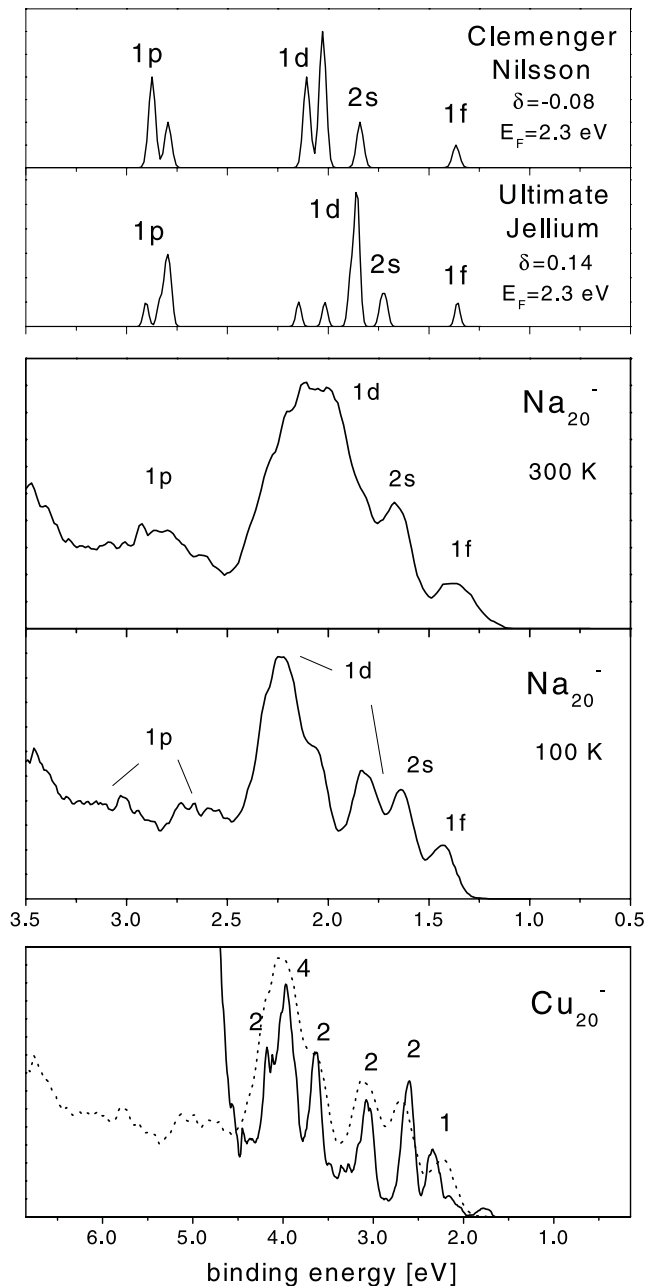
Fig. 1. Photoelectron spectra of hot and cold \text{Na}_{20}^- (with temperatures of 300 K and 100 K), measured at a photon energy of 4.02 eV, and of room temperature \text{Cu}_{20}^- , measured at a photon energy of 6.42 eV. The energy axes have been scaled according to the ratio of the bulk Fermi energies ( E_F(\text{Cu})/E_F(\text{Na}) = 2.23 ). In the sodium spectra the visible electron shells are identified by their quantum numbers; in the copper spectrum the numbers of electrons probably occupying each state have been indicated. Additionally the DOS as obtained from the Clemenger/Nilsson model [4] and from the “ultimate jellium” model [20] are shown. In both cases the total bandwidth (the energy interval between the shells 1s and 1f) has been chosen as 2.3 eV, which gave the best fit to the observed peak structure. Note that the Clemenger model predicts an oblate deformation of the cluster, while the ultimate jellium predicts a dominantly prolate one. Nevertheless both models fail to reproduce the observed spectrum.
