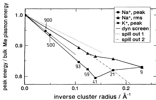
FIG. 2. Normalized peak positions for spherical \text{Na}_j^+ and large \text{K}_j^+ , as well as the root mean square [rms, see Eq. (2)] excitation energies of \text{Na}_j^+ are plotted against the inverse cluster radius. For j \geq 41 the peak and the rms energies extrapolate linearly to the Mie plasmon. The experimental slopes are in agreement with the predictions of the dynamic screening theory of surface science [Eq. (5)] and the spill-out equation of cluster science [Eq. (4)].
