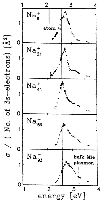
FIG. 1. Optical response of spherical sodium cluster ions. One large maximum is observed, accompanied by a shoulder on the high energy side. The vertical line gives the peak position for j = 41 , indicating the blueshift for smaller and larger clusters. The positions of the atomic and the Mie resonance are also indicated.
